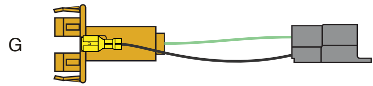
Back-up Light Socket & Pigtails (2 pcs)
